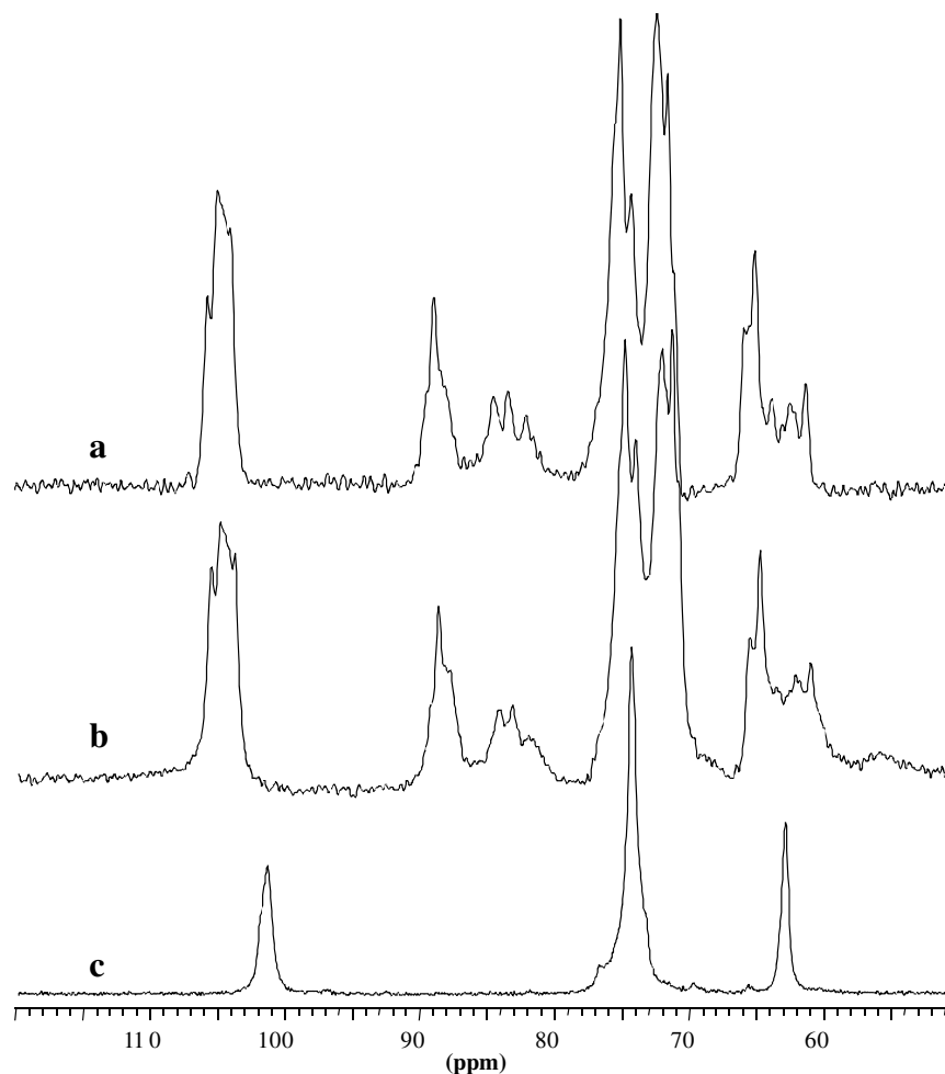
Fig. 9. CP/MAS ^{13}\text{C} NMR spectra of xylan or treated pericarp seed of OFI. (a) Aq. 6% NaOH – Residue IV; (b) aq. 6% NaOH – Gaulin Residue V-G; (c) 6% NaOH extracted xylan.
